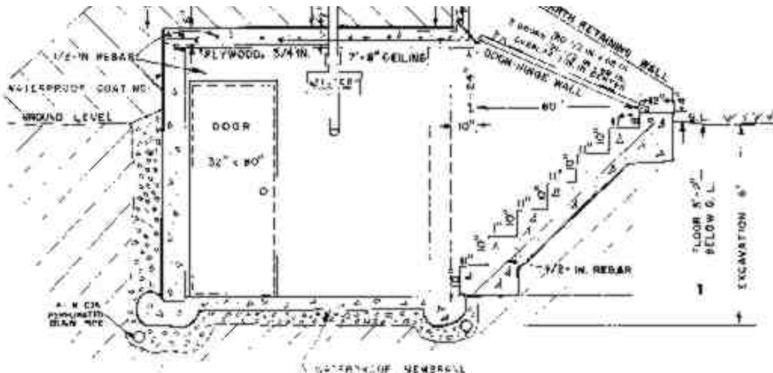
Fig. 17.1. Permanent Family Fallout Shelter for Dual Use.
