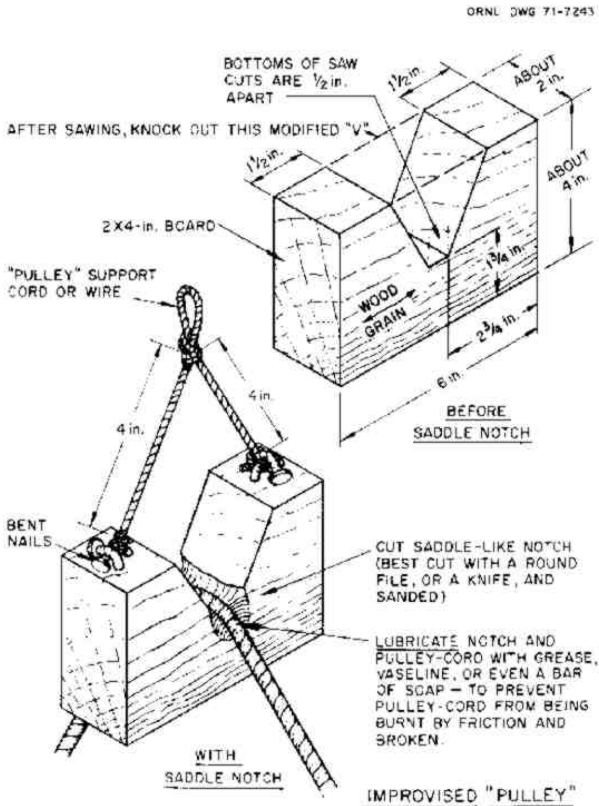
Fig. 18. IMPROVISED "PULLEY" ORNL DWG 71-7243
