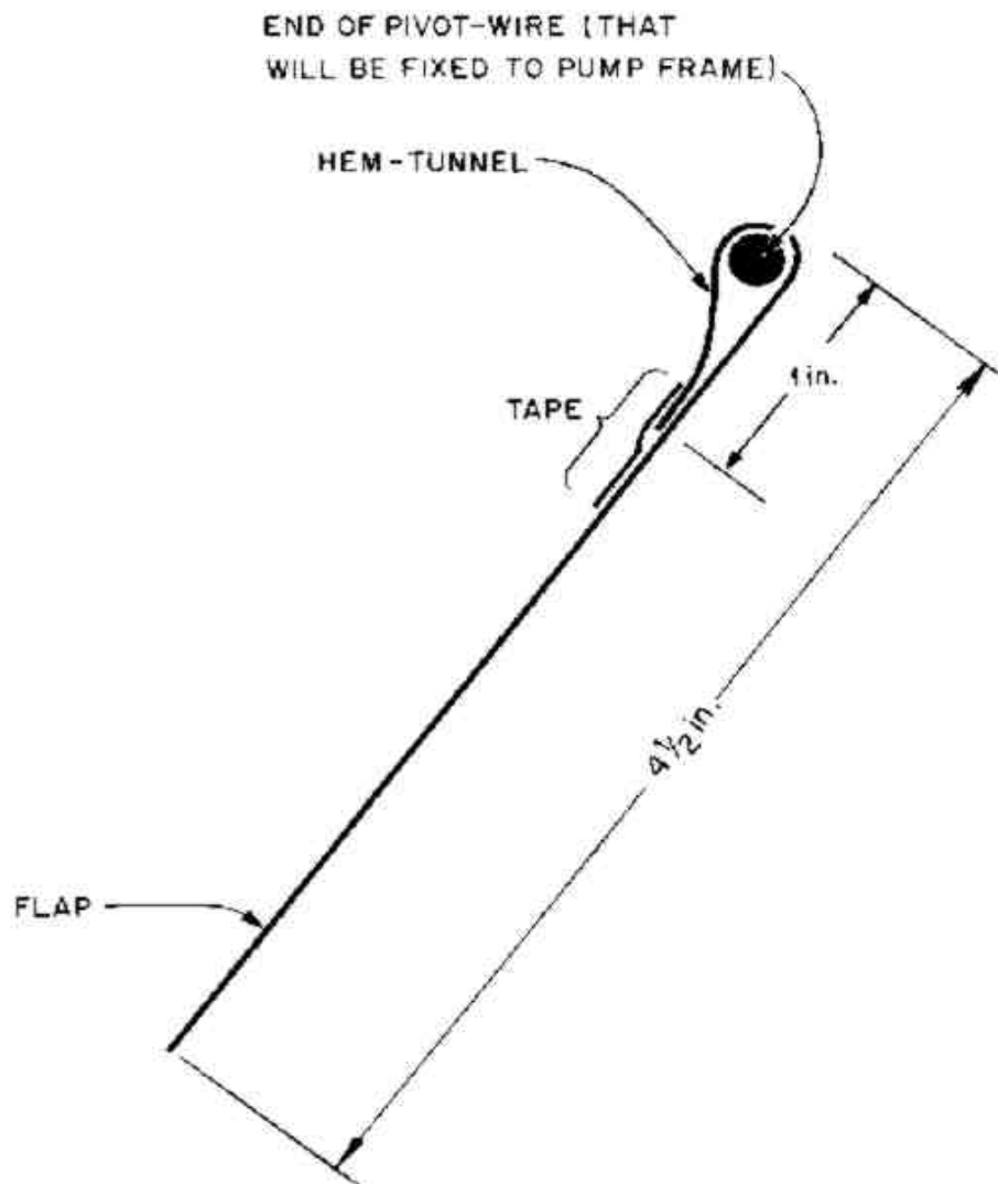
Fig. 7. End view.
