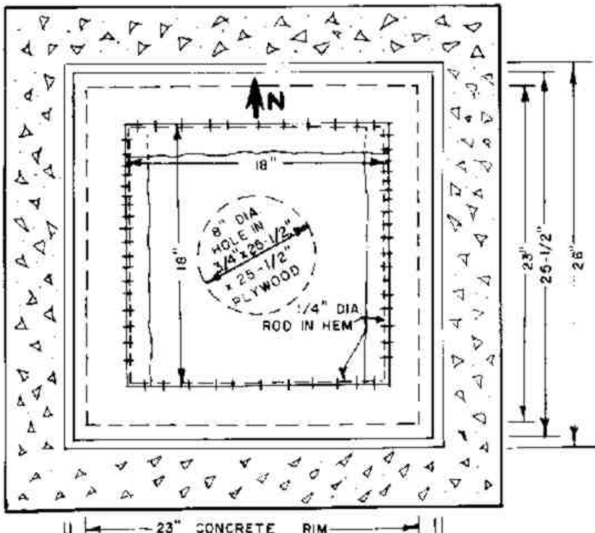
Fig. 17.3. Plan of Vertical Emergency Exit, Before Filling with Sand.
