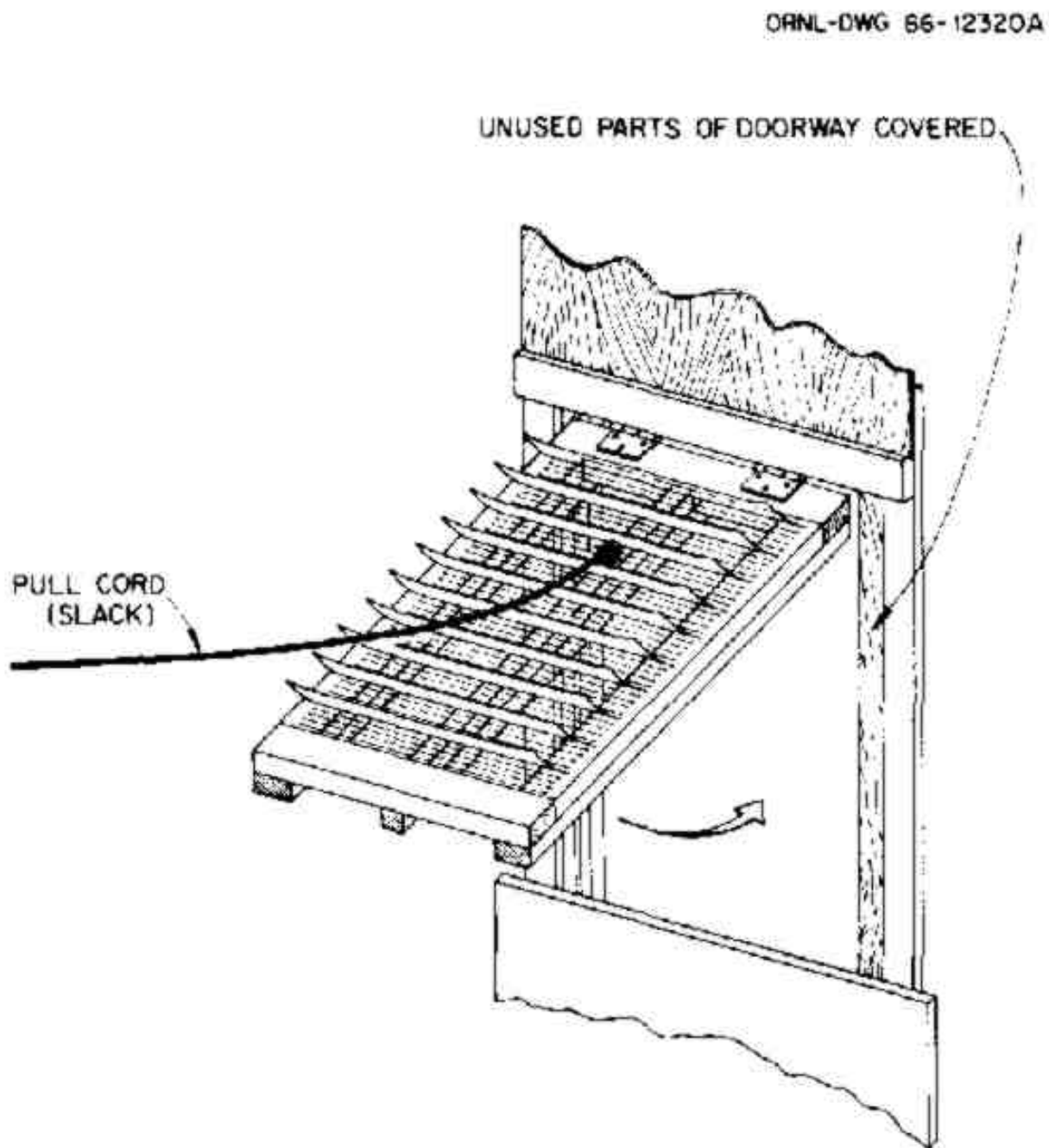
Fig. 1. Section through the upper part of a doorway, showing operation of a KAP. (ORNL-DWG 66-12320A)
