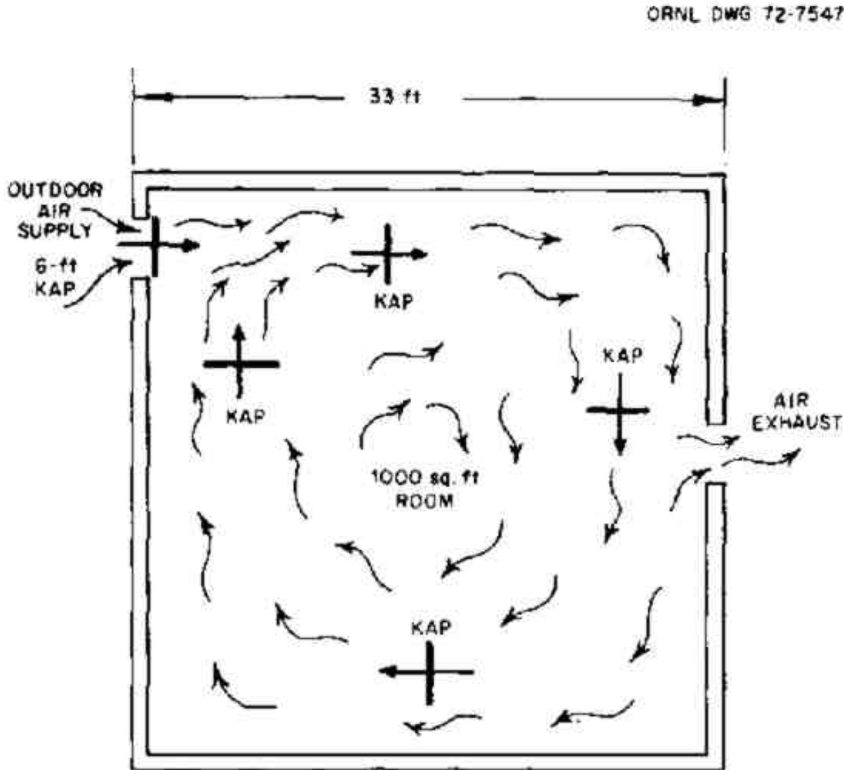
Fig. 16. The use of air-distribution KAPs.
