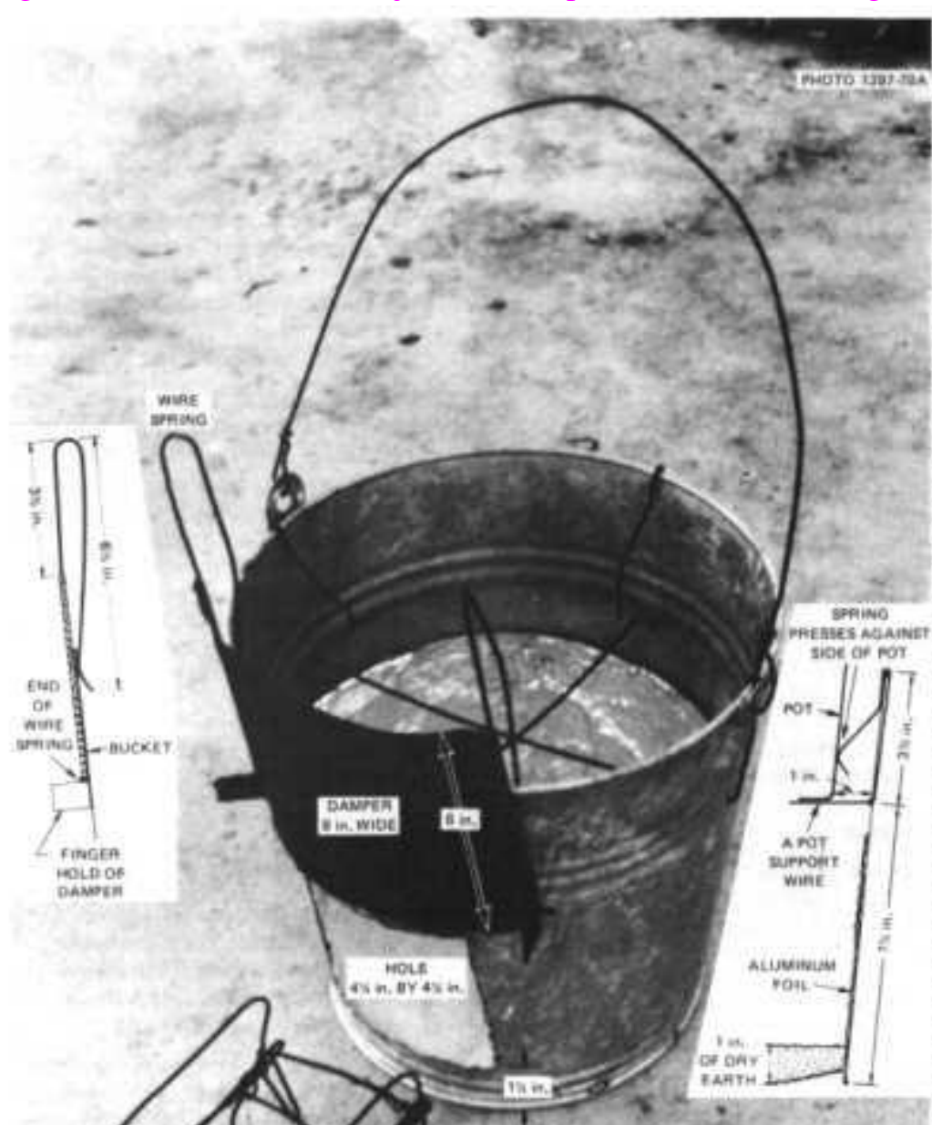
Fig. 9.2. Bucket-stove with adjustable damper and movable wire grate. Photo 1397-78A
