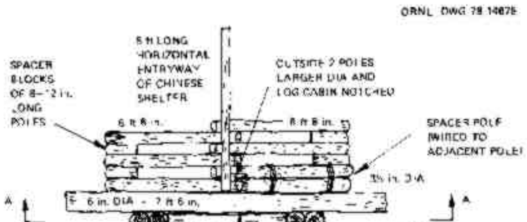
Fig. D. 11. Lower part of a vertical triangular entry, showing its connection to the horizontal part of the shelter entry. (ORNL-DWG 78-14675)
