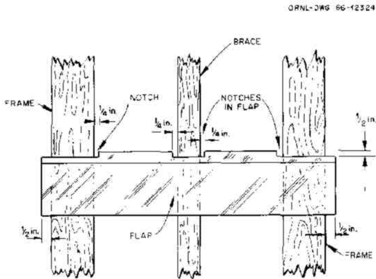
Fig. 6. Sizes of notches in flaps. ORNL-DWG 66-12324
