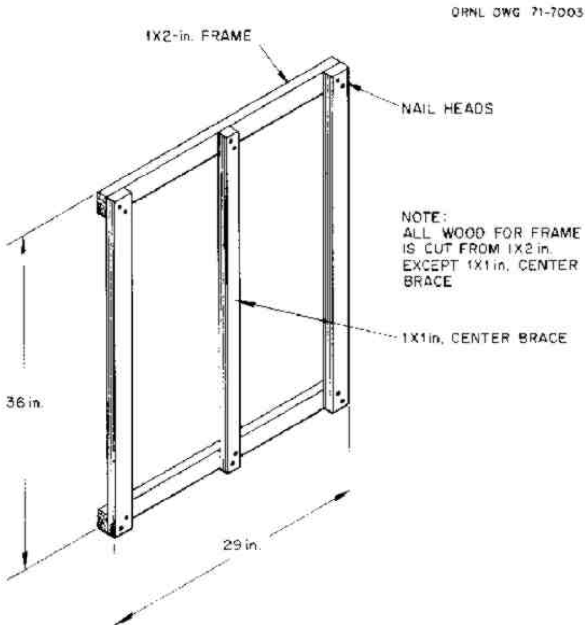
Fig. 3. KAP frame (looking at the back side of the frame). ORNL 71-7003
