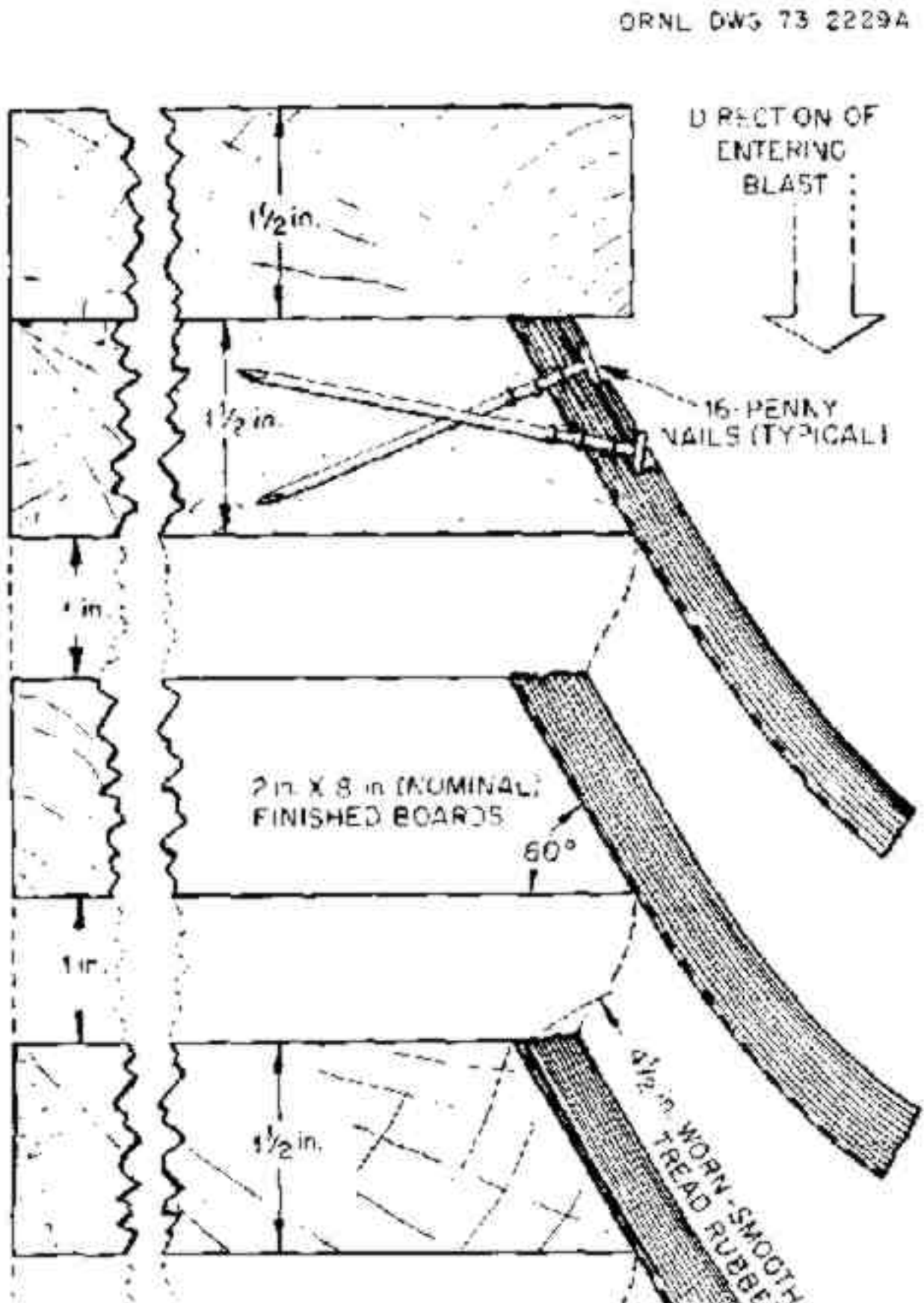
Fig. D.18. Overlapping-Flaps Blast Valve, made of boards, plywood, and strips cut from the treads of worn car tires. (ORNL DWG 73-2229A)
