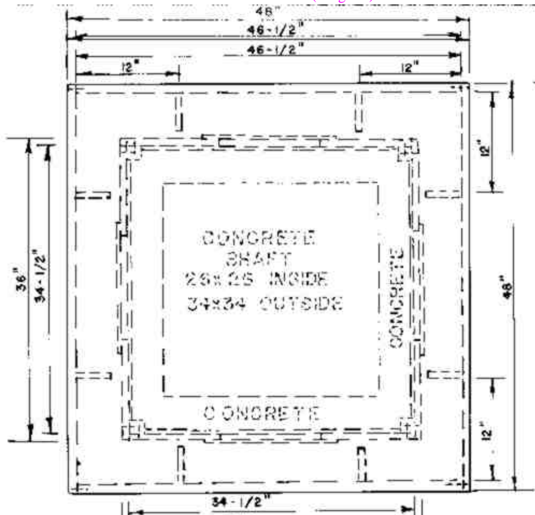
Fig. F.2. Plan and Side View of Multi- Purpose Emergency Exit Housing, on a Square Emergency Exit with 34 x 34-Inch Cross- Sectional Outside Dimensions. (Diagram)
